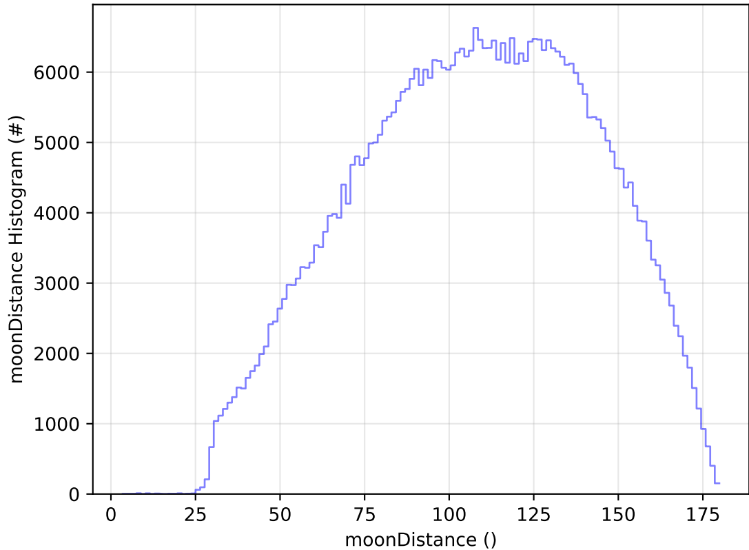
too_combined_no_nss_s10.0_v3.4_10yrs All sky r band: moonDistance Histogram
