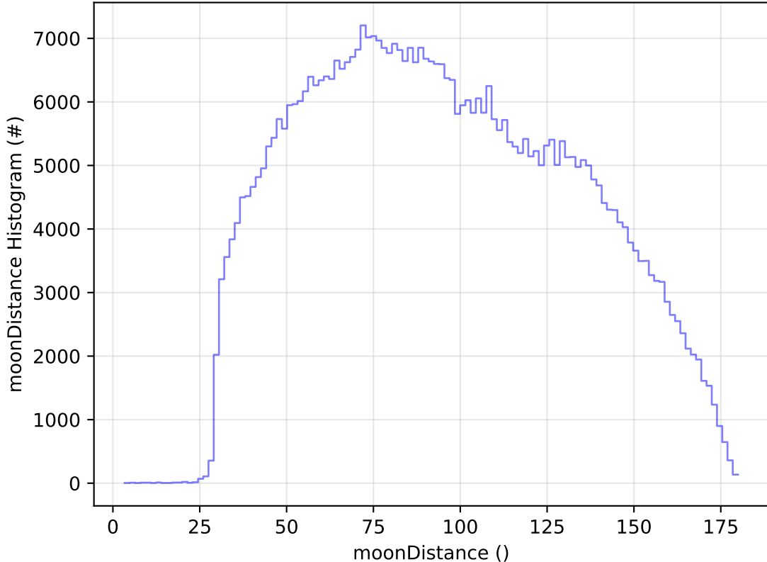
too_combined_no_nss_s10.0_v3.4_10yrs All sky i band: moonDistance Histogram
