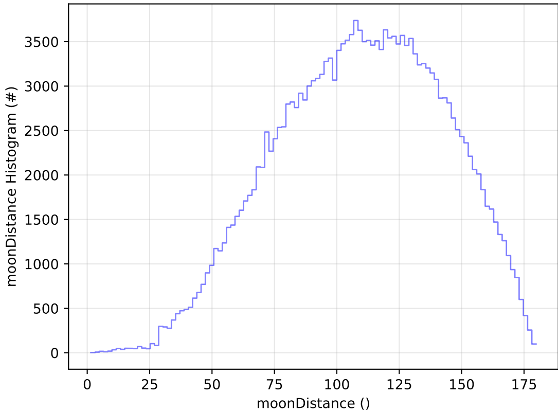
too_combined_no_nss_s10.0_v3.4_10yrs All sky g band: moonDistance Histogram
