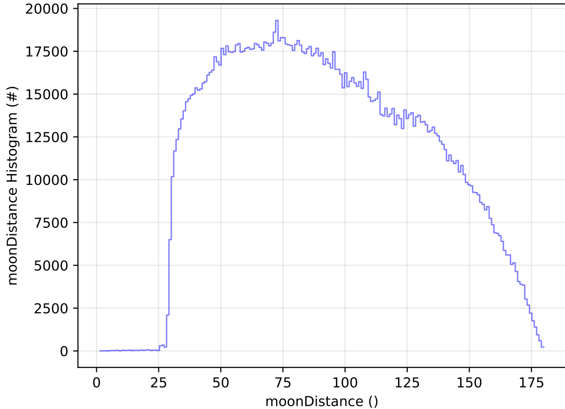
too_combined_no_nss_s10.0_v3.4_10yrs All sky all bands: moonDistance Histogram
