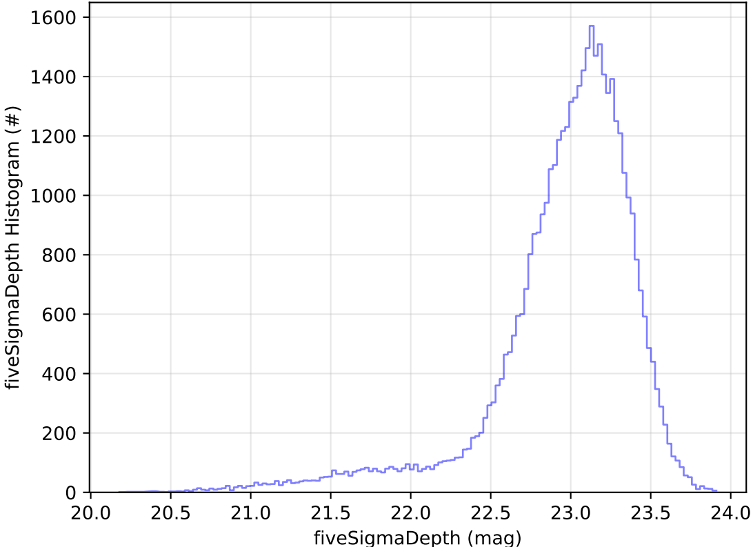
too_combined_no_nss_s10.0_v3.4_10yrs Yr 1 z band: fiveSigmaDepth Histogram
