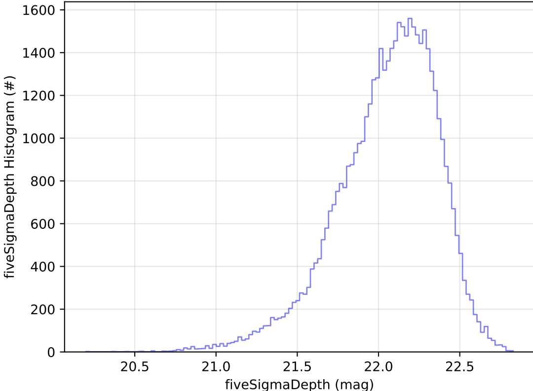
too_combined_no_nss_s10.0_v3.4_10yrs Yr 1 y band: fiveSigmaDepth Histogram
