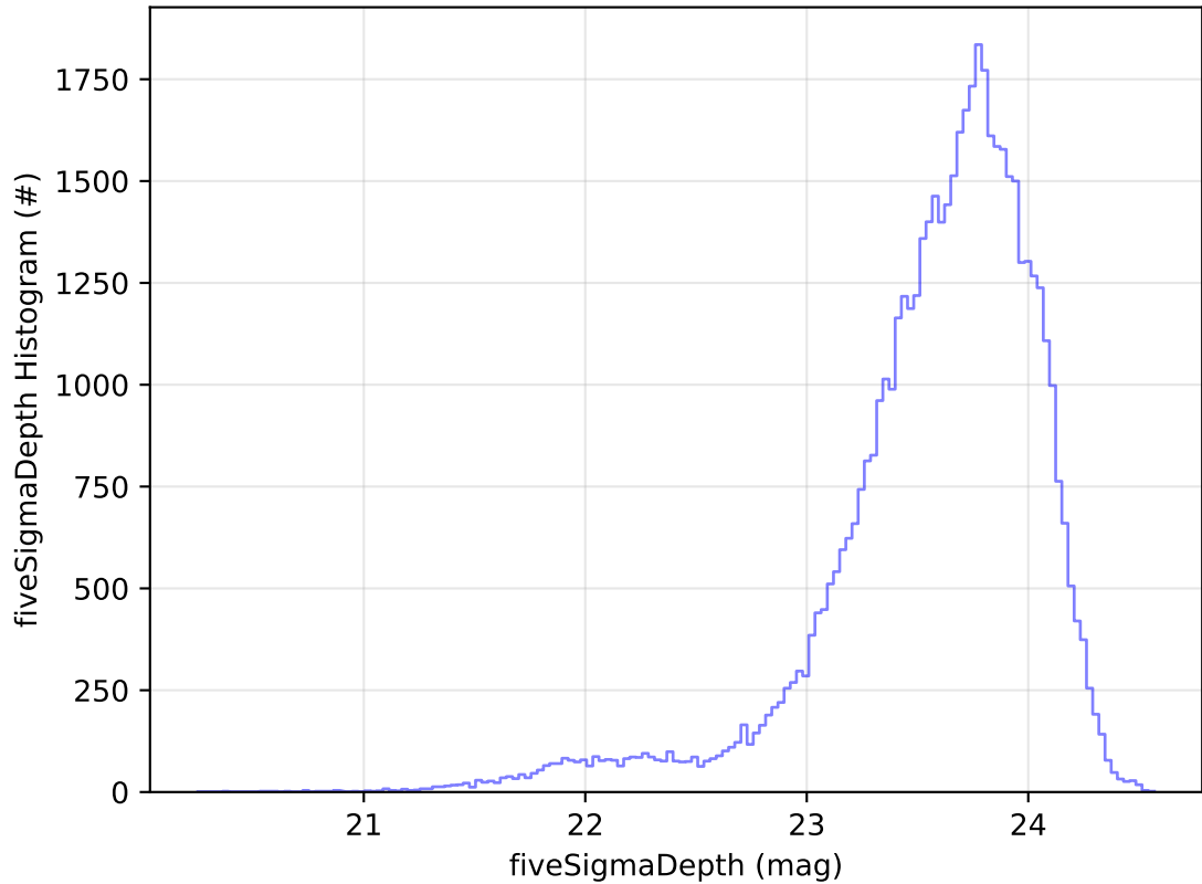
too_combined_no_nss_s10.0_v3.4_10yrs Yr 1 i band: fiveSigmaDepth Histogram
