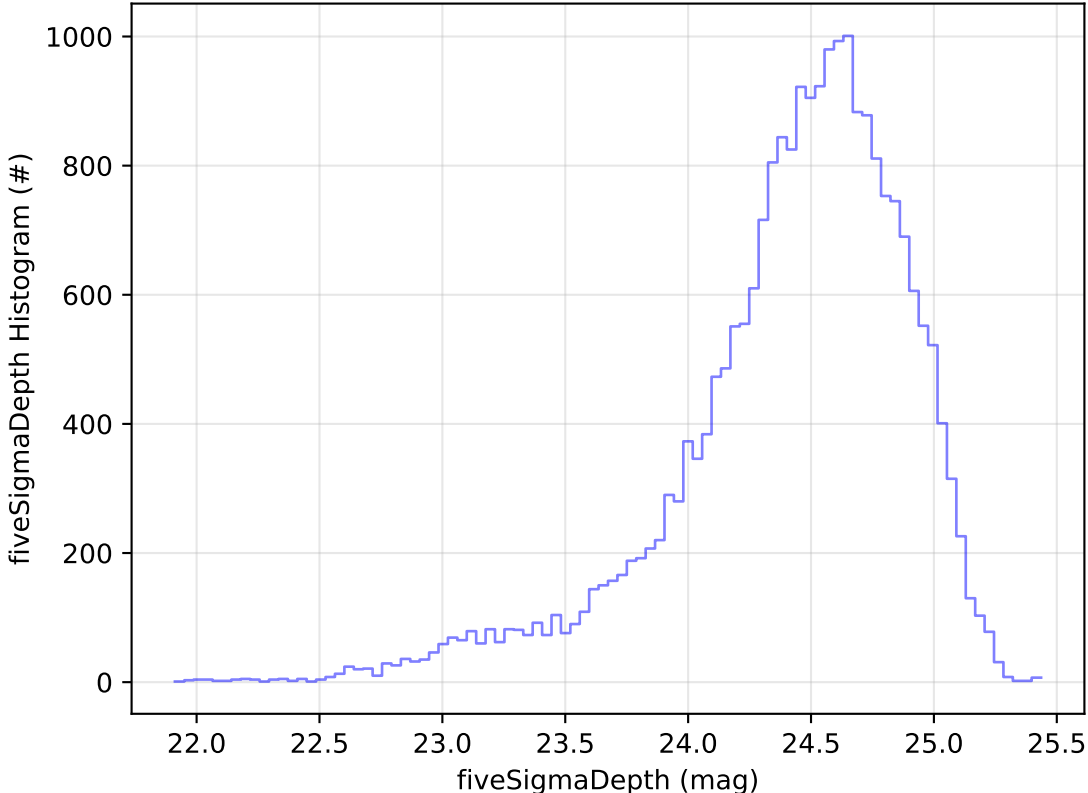
too_combined_no_nss_s10.0_v3.4_10yrs Yr 1 g band: fiveSigmaDepth Histogram
