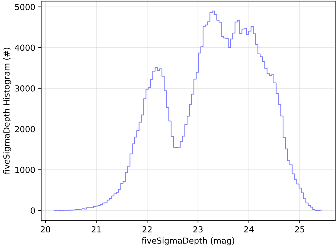
too_combined_no_nss_s10.0_v3.4_10yrs Yr 1 all bands: fiveSigmaDepth Histogram
