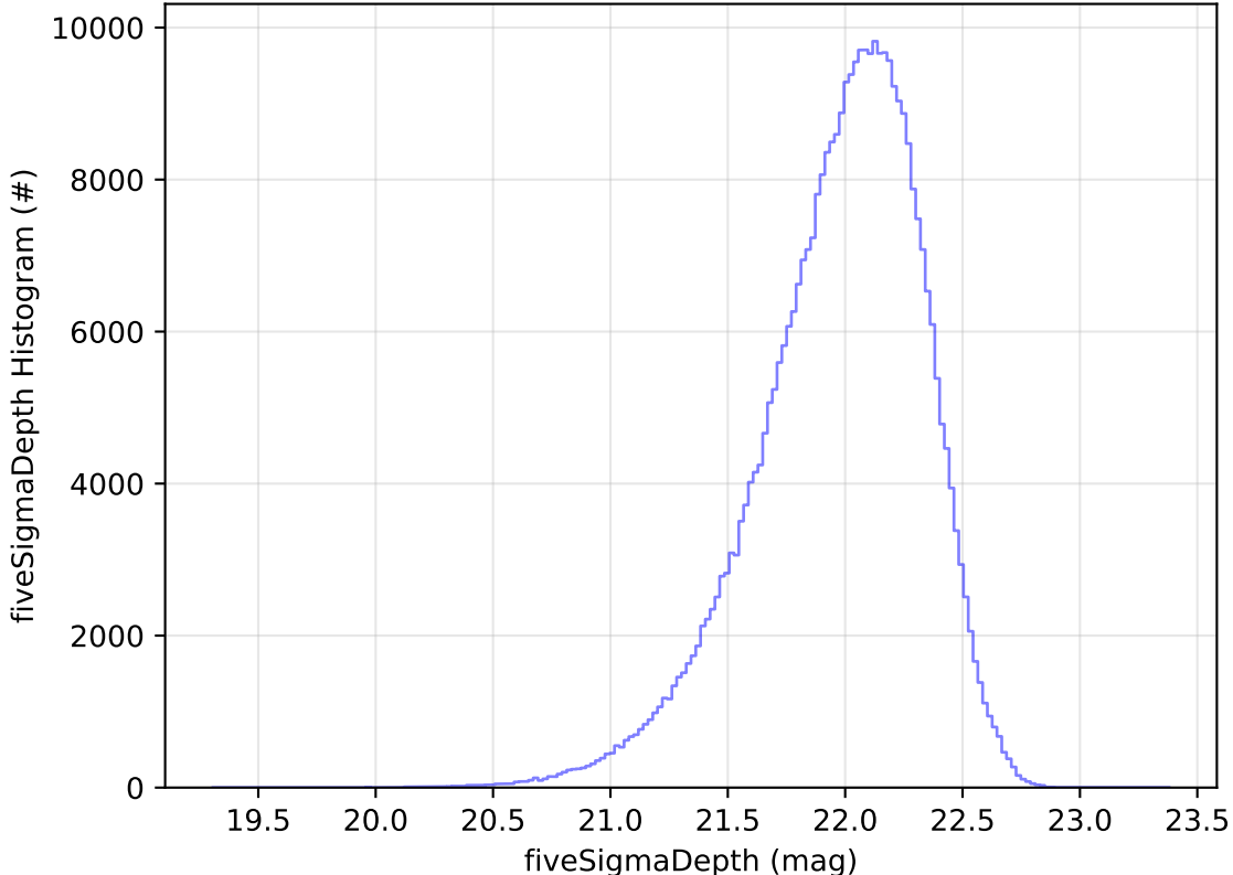
too_combined_no_nss_s10.0_v3.4_10yrs WFD y band: fiveSigmaDepth Histogram
