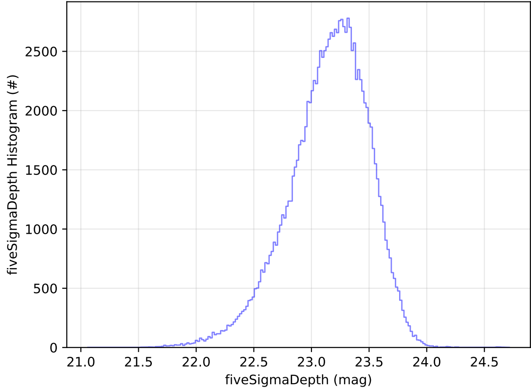
too_combined_no_nss_s10.0_v3.4_10yrs WFD u band: fiveSigmaDepth Histogram
