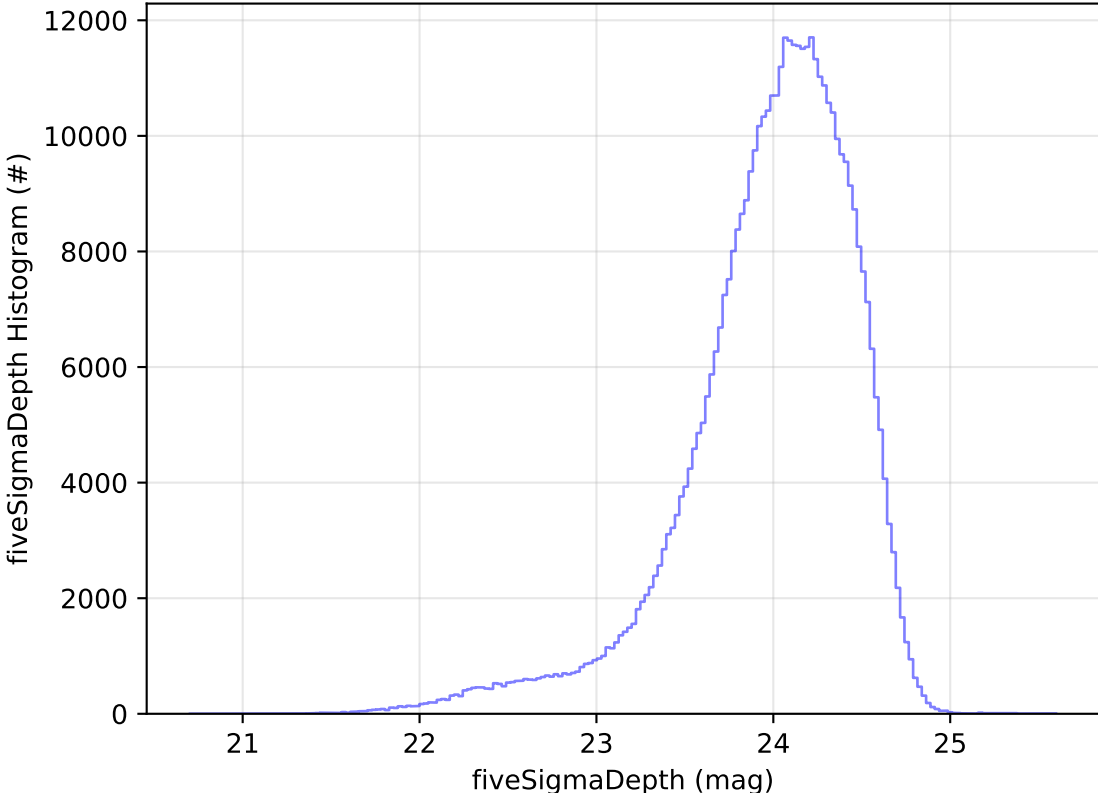
too_combined_no_nss_s10.0_v3.4_10yrs WFD r band: fiveSigmaDepth Histogram
