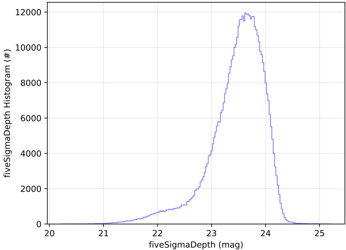
too_combined_no_nss_s10.0_v3.4_10yrs WFD i band: fiveSigmaDepth Histogram
