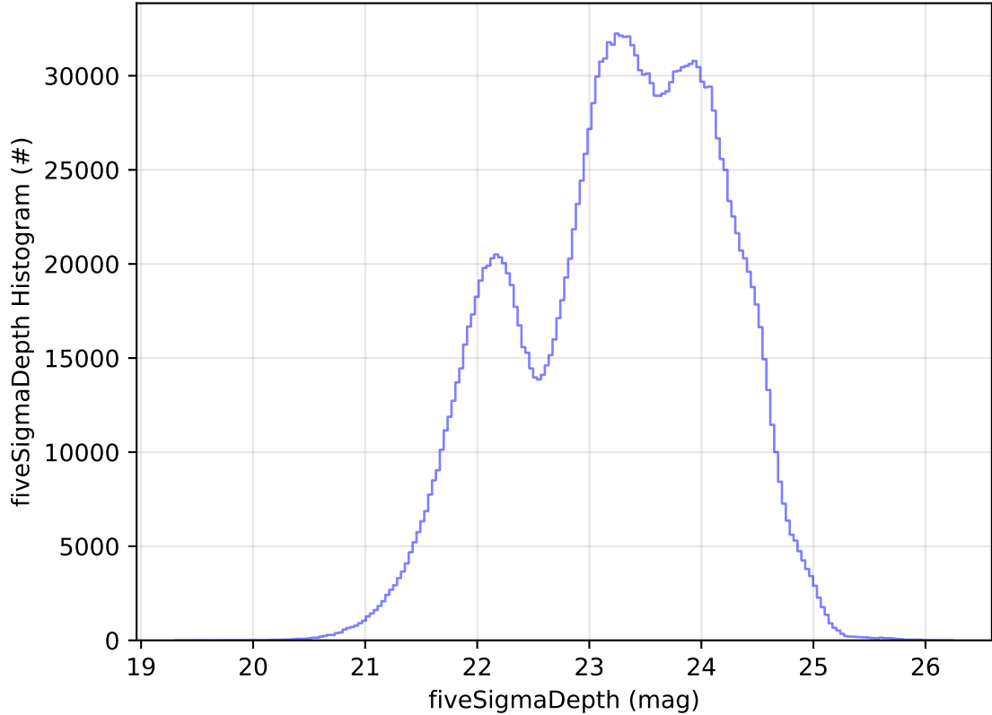
too_combined_no_nss_s10.0_v3.4_10yrs WFD all bands: fiveSigmaDepth Histogram
