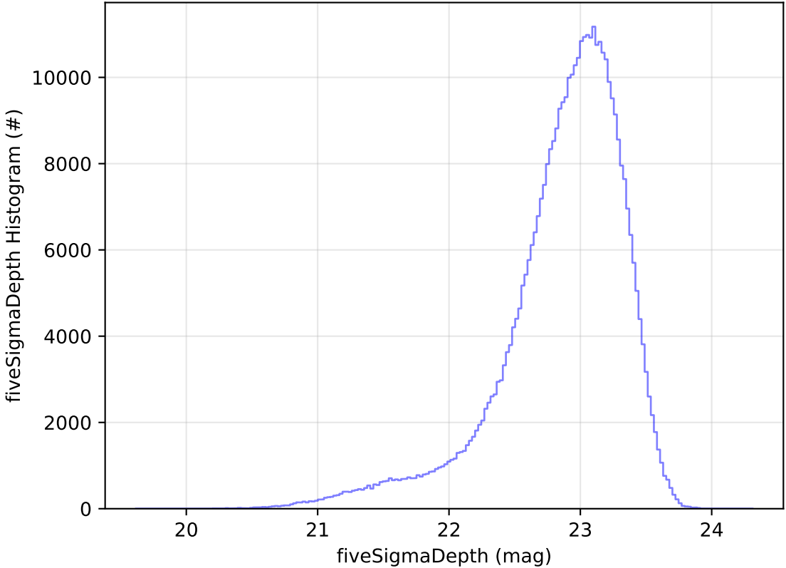
too_combined_no_nss_s10.0_v3.4_10yrs All sky z band: fiveSigmaDepth Histogram
