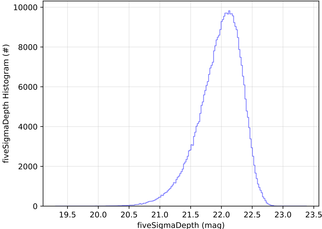
too_combined_no_nss_s10.0_v3.4_10yrs All sky y band: fiveSigmaDepth Histogram
