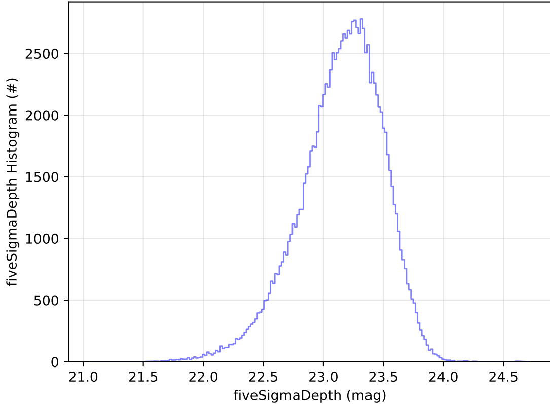
too_combined_no_nss_s10.0_v3.4_10yrs All sky u band: fiveSigmaDepth Histogram
