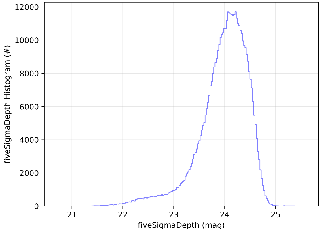
too_combined_no_nss_s10.0_v3.4_10yrs All sky r band: fiveSigmaDepth Histogram
