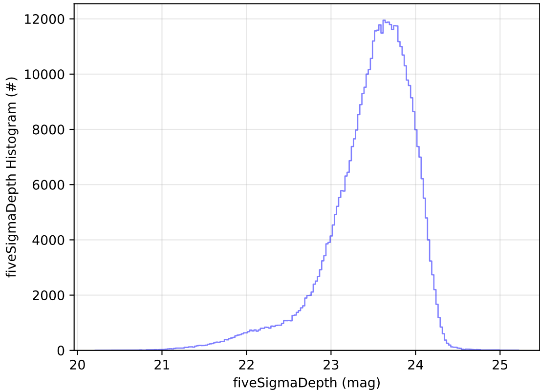
too_combined_no_nss_s10.0_v3.4_10yrs All sky i band: fiveSigmaDepth Histogram
