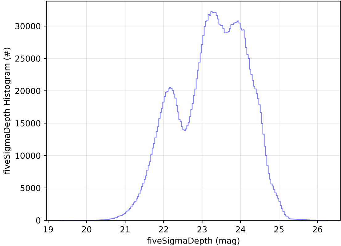
too_combined_no_nss_s10.0_v3.4_10yrs All sky all bands: fiveSigmaDepth Histogram
