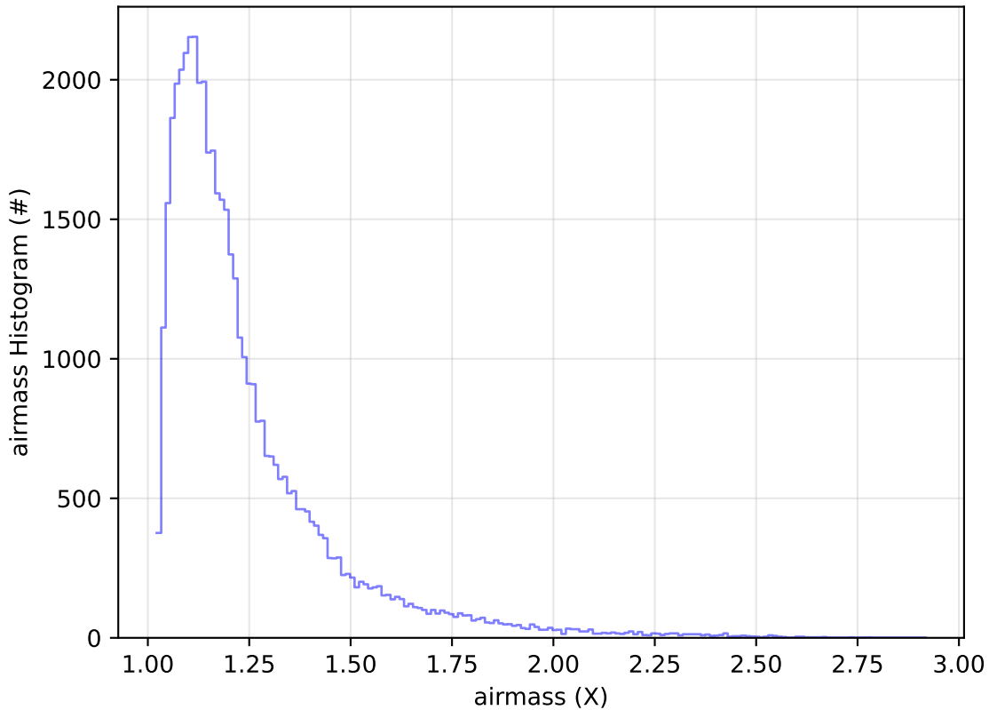
too_combined_no_nss_s10.0_v3.4_10yrs Yr 1 y band: airmass Histogram
