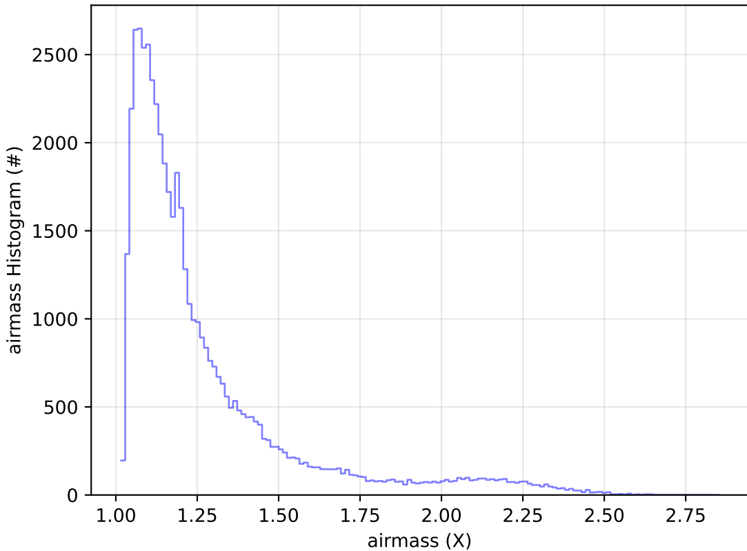
too_combined_no_nss_s10.0_v3.4_10yrs Yr 1 r band: airmass Histogram
