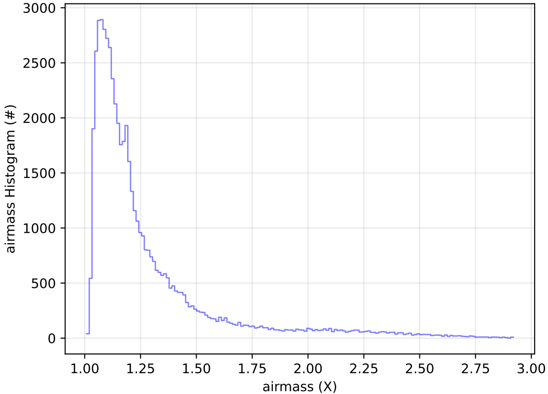
too_combined_no_nss_s10.0_v3.4_10yrs Yr 1 i band: airmass Histogram
