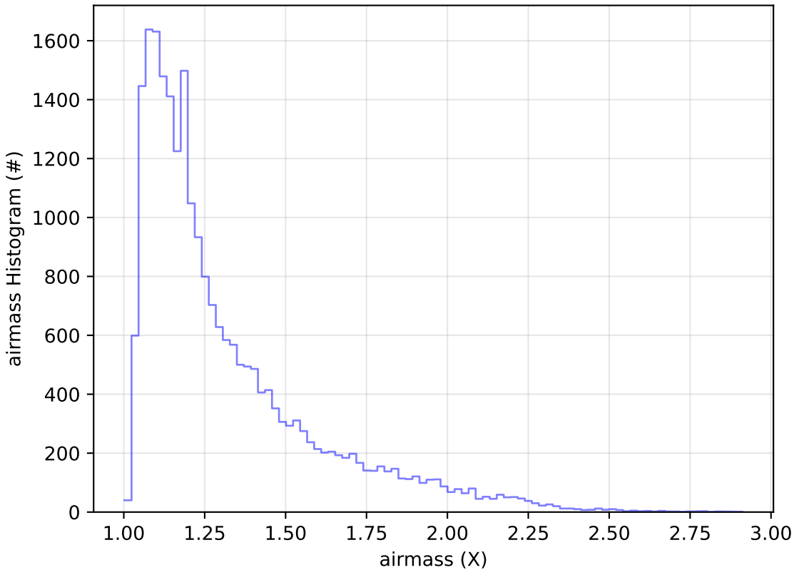
too_combined_no_nss_s10.0_v3.4_10yrs Yr 1 g band: airmass Histogram
