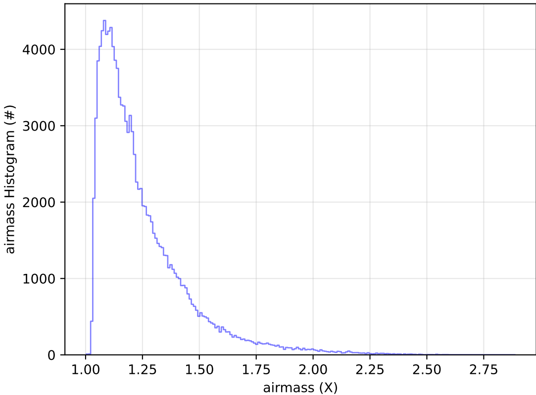
too_combined_no_nss_s10.0_v3.4_10yrs WFD u band: airmass Histogram
