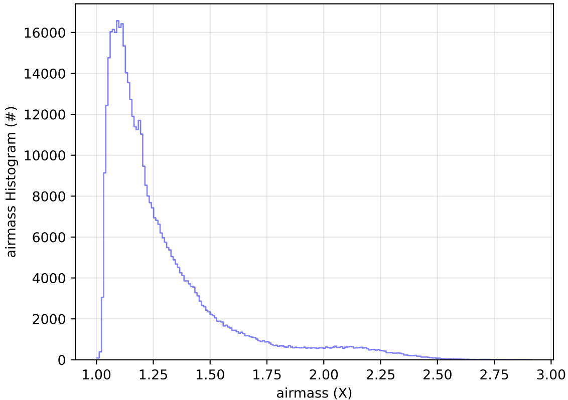
too_combined_no_nss_s10.0_v3.4_10yrs WFD r band: airmass Histogram
