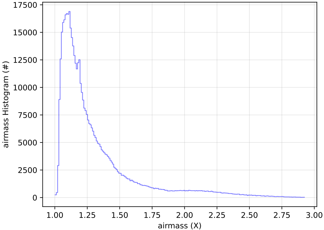
too_combined_no_nss_s10.0_v3.4_10yrs WFD i band: airmass Histogram
