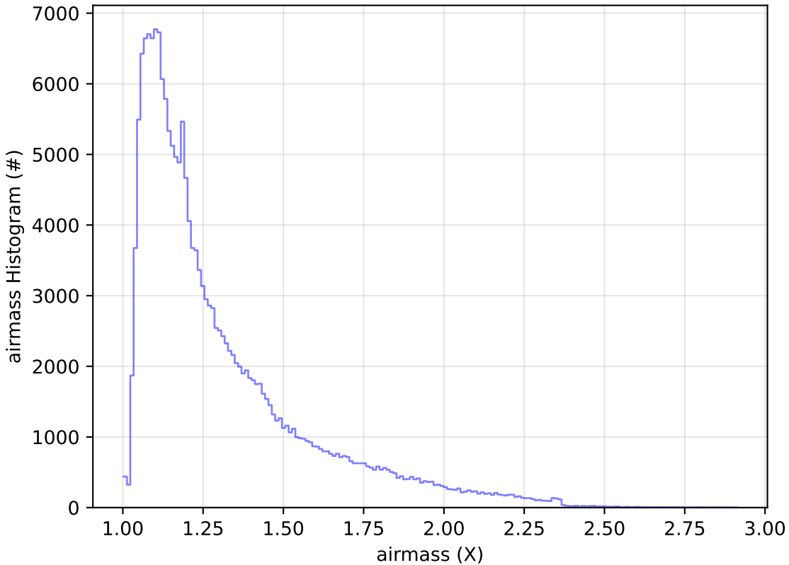
too_combined_no_nss_s10.0_v3.4_10yrs WFD g band: airmass Histogram
