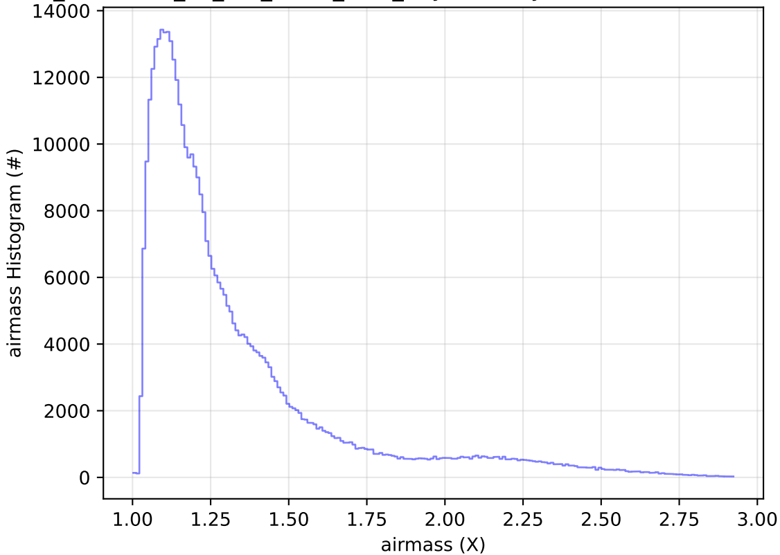
too_combined_no_nss_s10.0_v3.4_10yrs All sky z band: airmass Histogram
