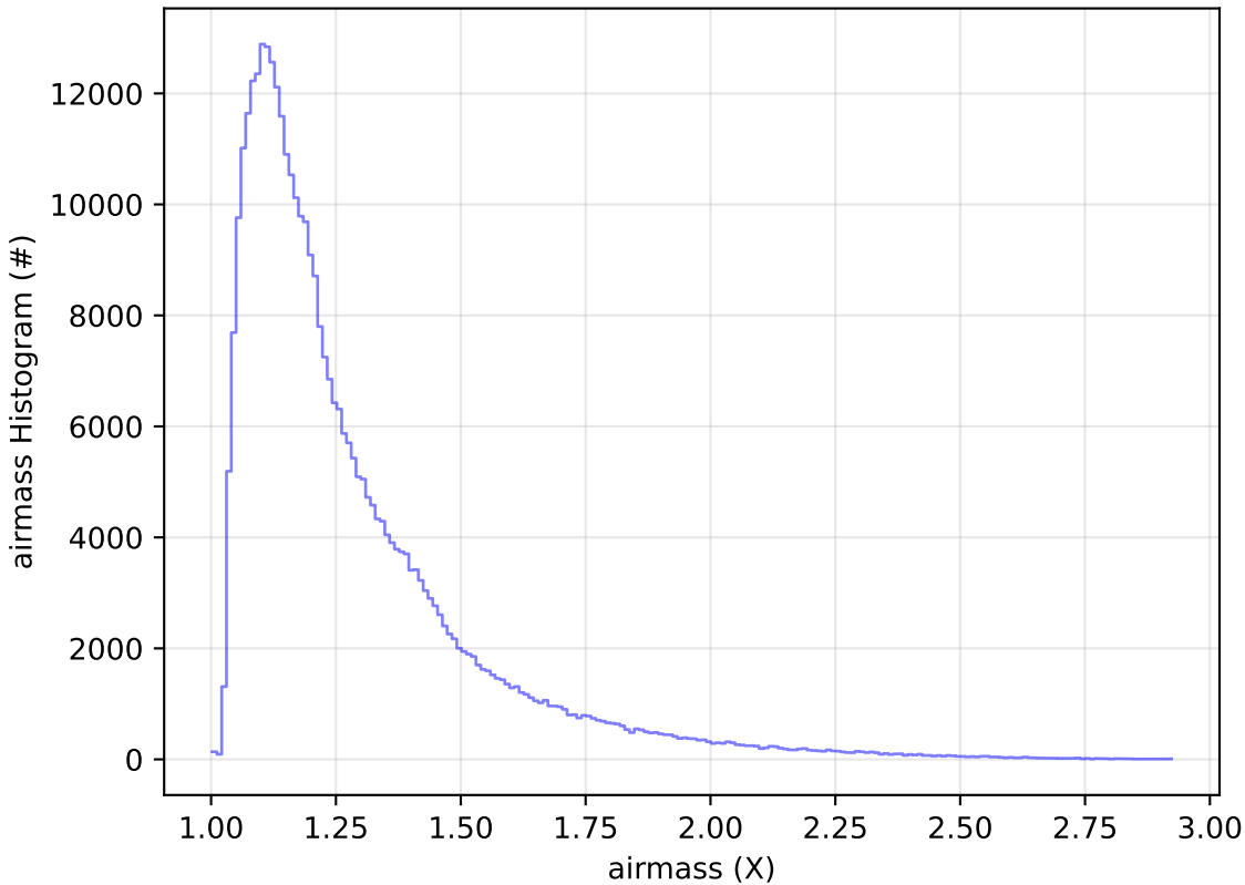
too_combined_no_nss_s10.0_v3.4_10yrs All sky y band: airmass Histogram
