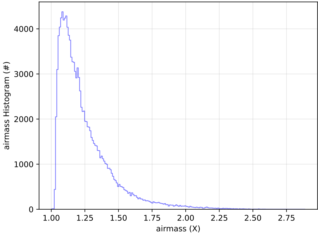
too_combined_no_nss_s10.0_v3.4_10yrs All sky u band: airmass Histogram
