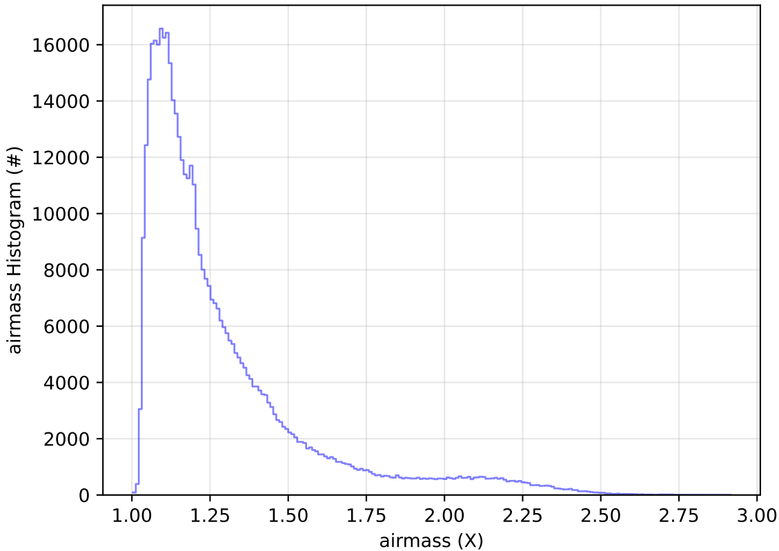
too_combined_no_nss_s10.0_v3.4_10yrs All sky r band: airmass Histogram
