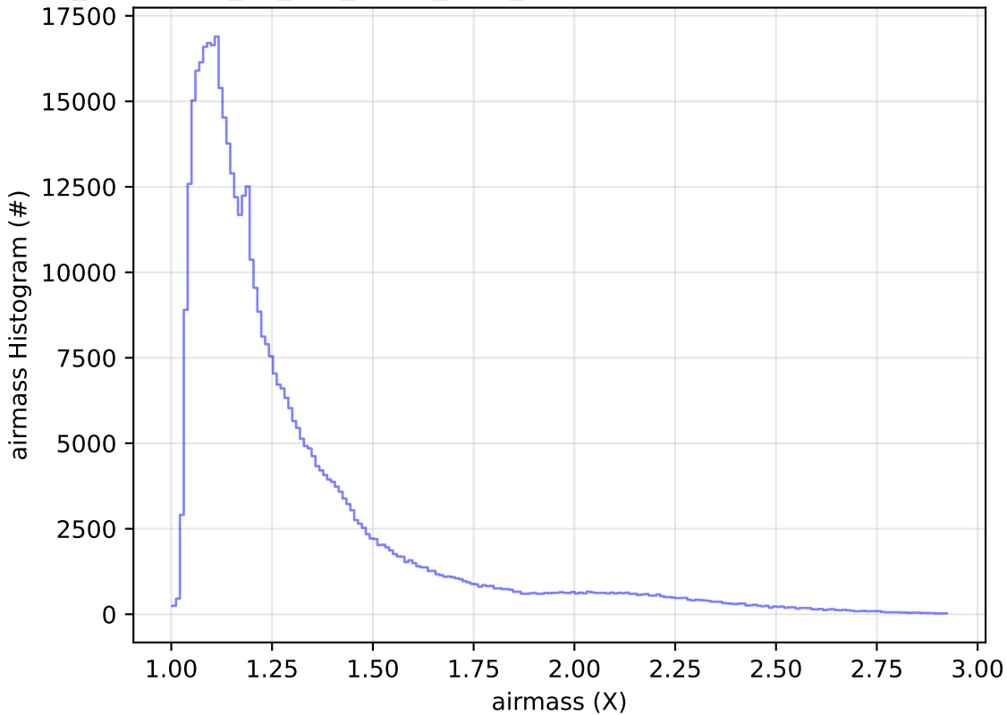
too_combined_no_nss_s10.0_v3.4_10yrs All sky i band: airmass Histogram
