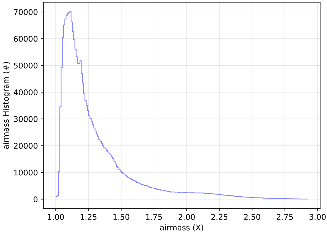
too_combined_no_nss_s10.0_v3.4_10yrs All sky all bands: airmass Histogram
