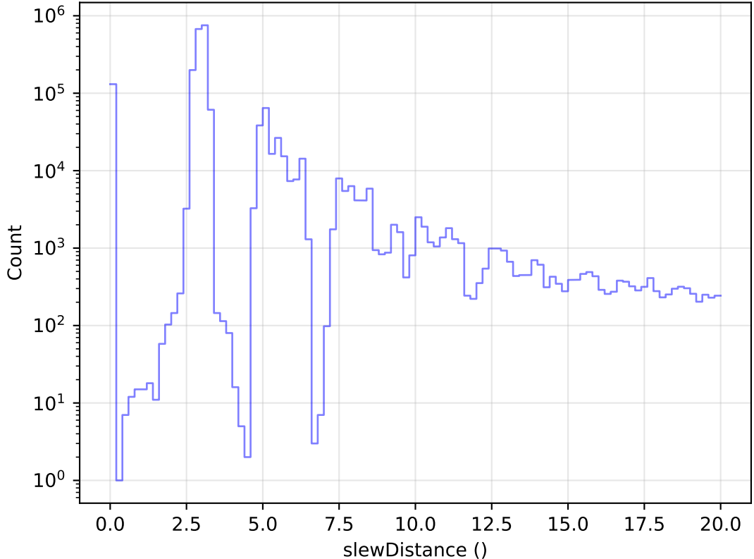
too_combined_no_nss_s10.0_v3.4_10yrs All visits: Zoom Slew Distance Histogram
