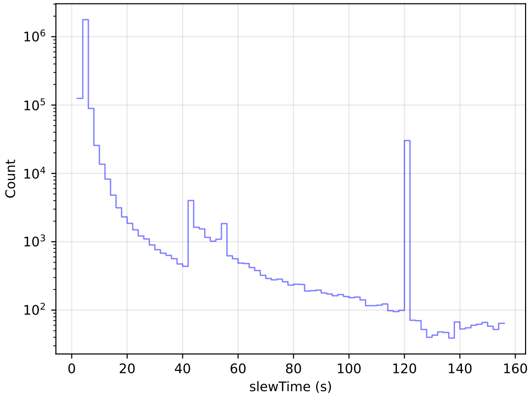
too_combined_no_nss_s10.0_v3.4_10yrs All visits: Slew Time Histogram
