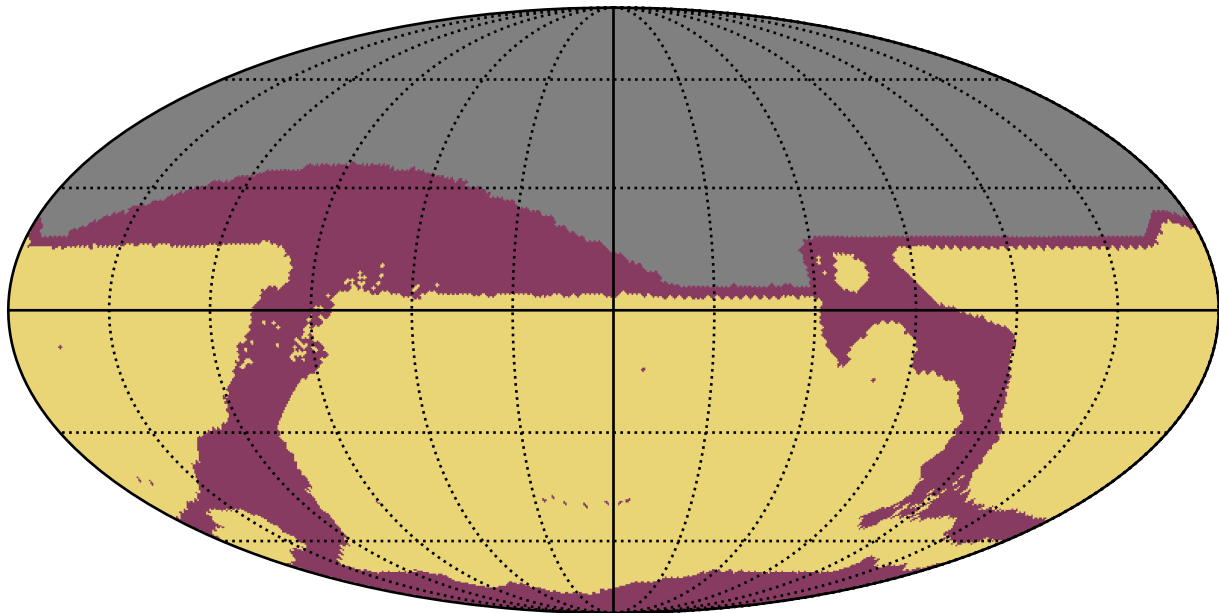
too_combined_no_nss_s10.0_v3.4_10yrs All sky: RapidRevisits
