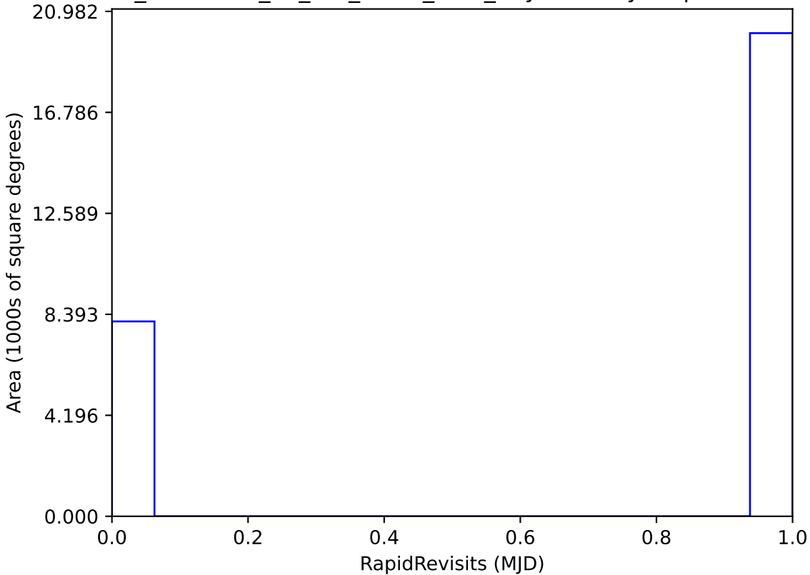
too_combined_no_nss_s10.0_v3.4_10yrs All sky: RapidRevisits
