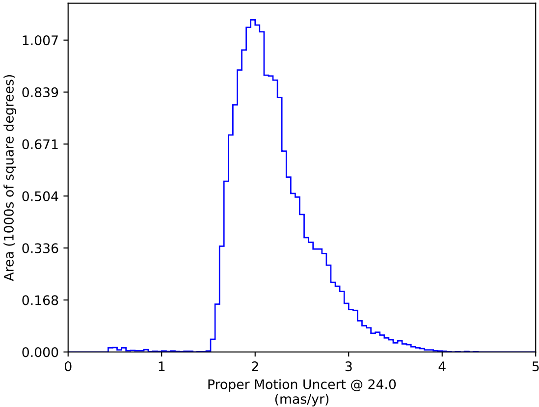
too_combined_no_nss_s10.0_v3.4_10yrs WFD: Proper Motion Uncert @ 24.0
