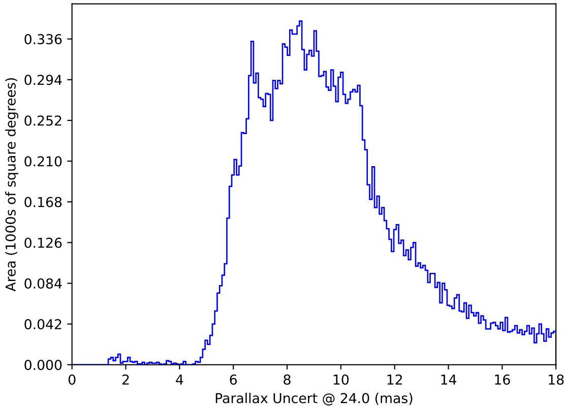
too_combined_no_nss_s10.0_v3.4_10yrs All sky: Parallax Uncert @ 24.0
