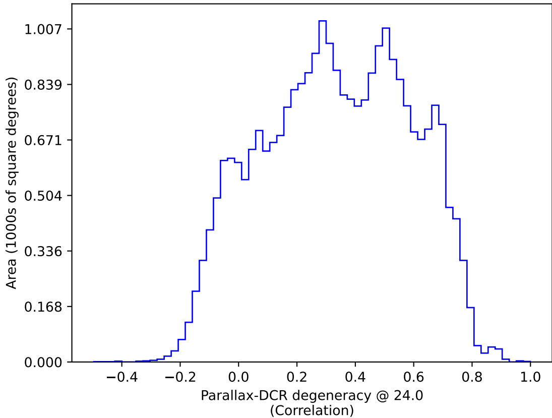
too_combined_no_nss_s10.0_v3.4_10yrs All sky: Parallax-DCR degeneracy @ 24.0
