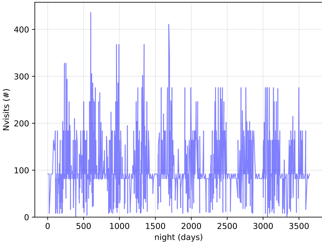
too_combined_no_nss_s10.0_v3.4_10yrs DDF: Nvisits
