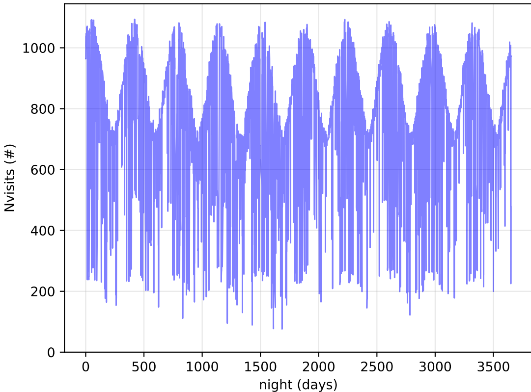
too_combined_no_nss_s10.0_v3.4_10yrs All visits: Nvisits
