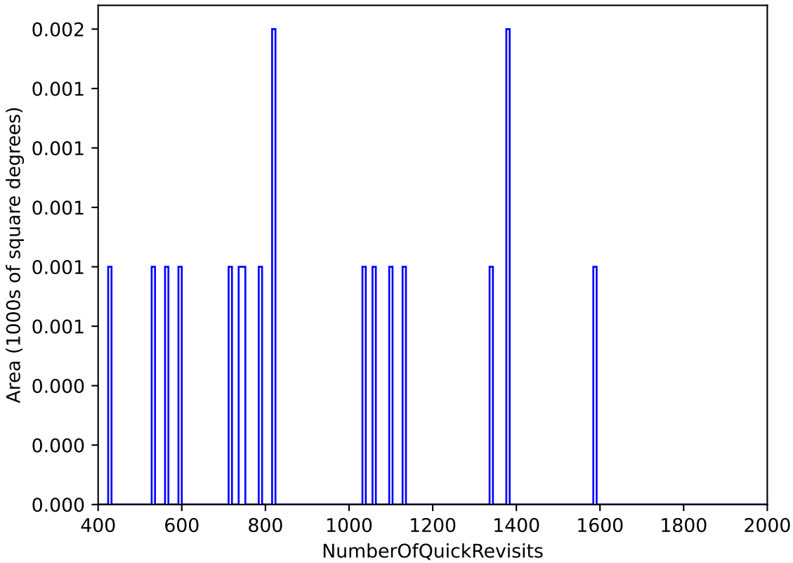
too_combined_no_nss_s10.0_v3.4_10yrs WFD: NumberOfQuickRevisits
