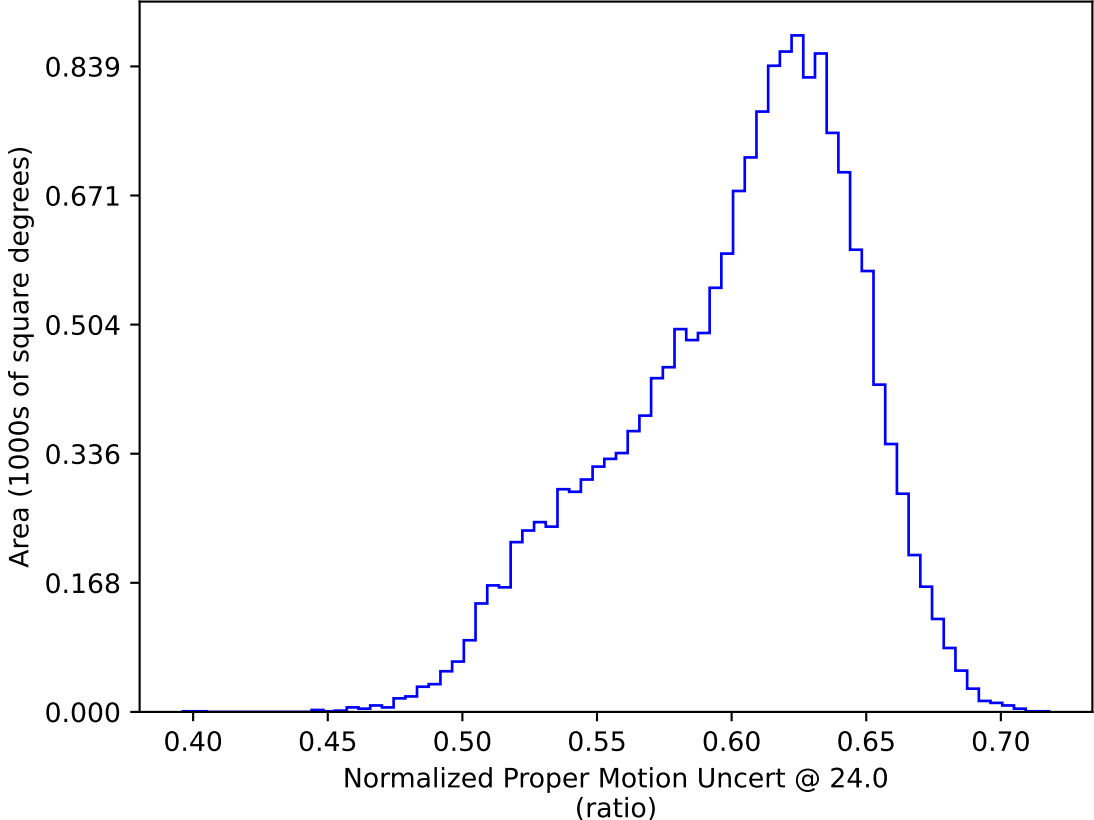
too_combined_no_nss_s10.0_v3.4_10yrs WFD: Normalized Proper Motion Uncert @ 24.0
