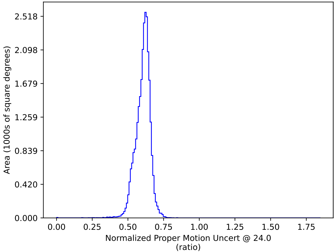
too_combined_no_nss_s10.0_v3.4_10yrs All sky: Normalized Proper Motion Uncert @ 24.0
