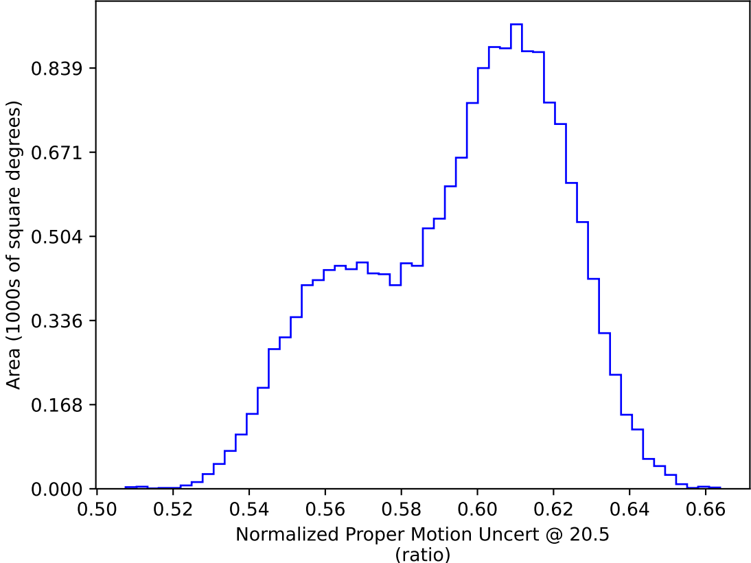
too_combined_no_nss_s10.0_v3.4_10yrs WFD: Normalized Proper Motion Uncert @ 20.5
