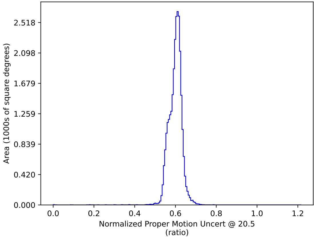
too_combined_no_nss_s10.0_v3.4_10yrs All sky: Normalized Proper Motion Uncert @ 20.5
