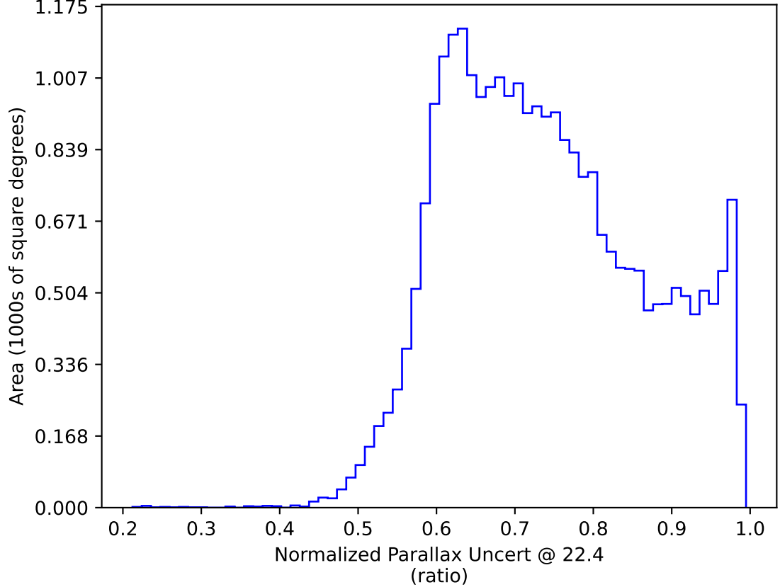
too_combined_no_nss_s10.0_v3.4_10yrs All sky: Normalized Parallax Uncert @ 22.4
