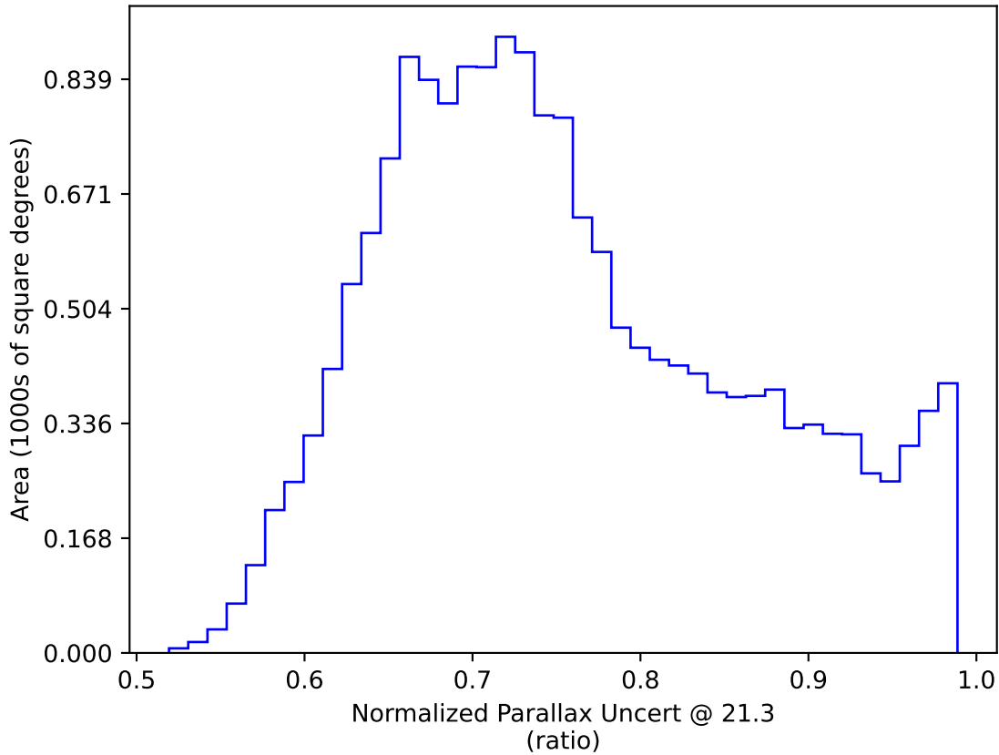
too_combined_no_nss_s10.0_v3.4_10yrs WFD y band only: Normalized Parallax Uncert @ 21.3
